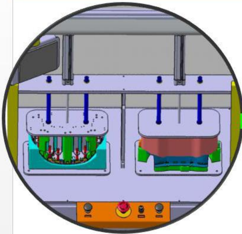
BJA CLUSTER FRAME ASSY MACHINE WITH POKA-YOKE
