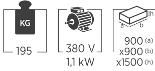
HKC 01 HAMUR KONİK ÇEVİRME MAKİNESİ CONICAL ROUNDING MACHINE
