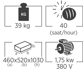
GLT 01 BAYAT EKMEK ÖĞÜTME MAKİNESİ BREAD CRUMBS MACHINE
