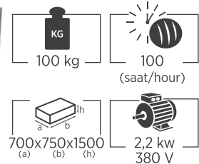
PM 01 PUDRA ŞEKERİ MAKİNESİ POWDERED SUGAR MACHINE
