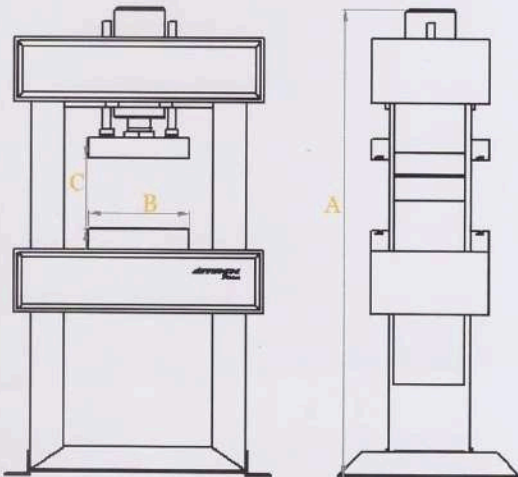
Technical Drawing
