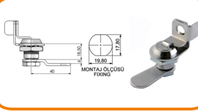
MANDALLI KİLİT EĞRİ DİLLİ (ASTHMA HAMİLLİ)
