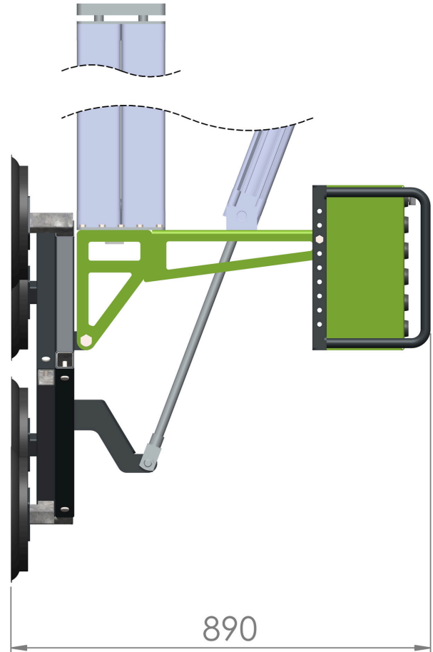
PVL-600VT-PL Lifting with pneumatic cylinder
