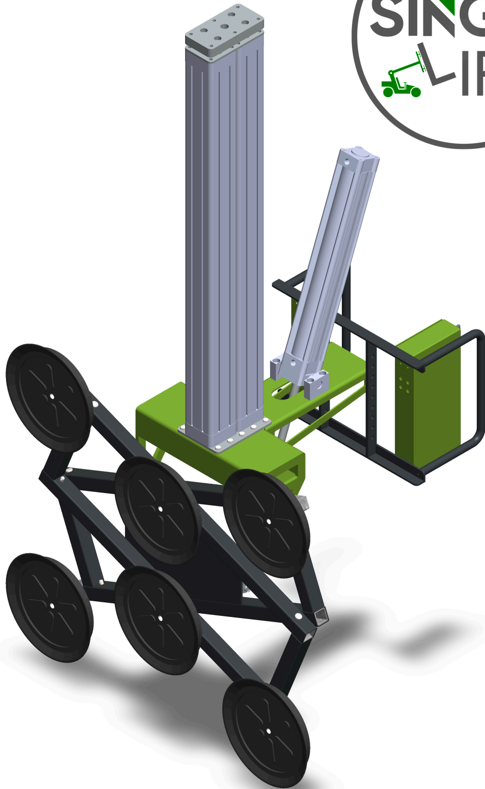
PVL-600VT-PL Lifting with pneumatic cylinder
