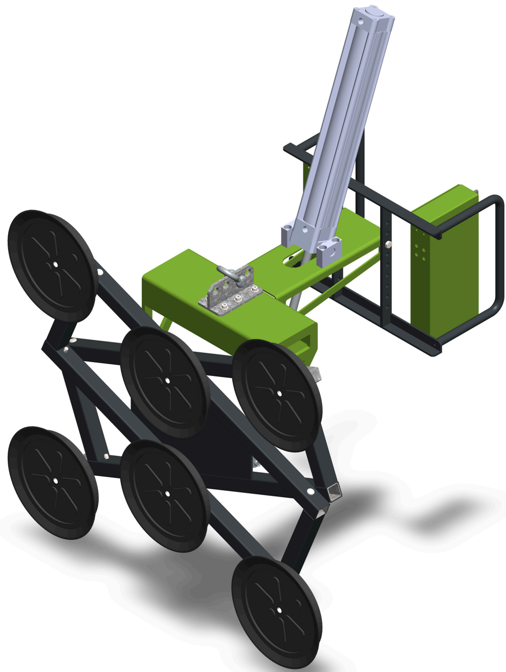
PVL-600VT-EW Lifting with electric winch
