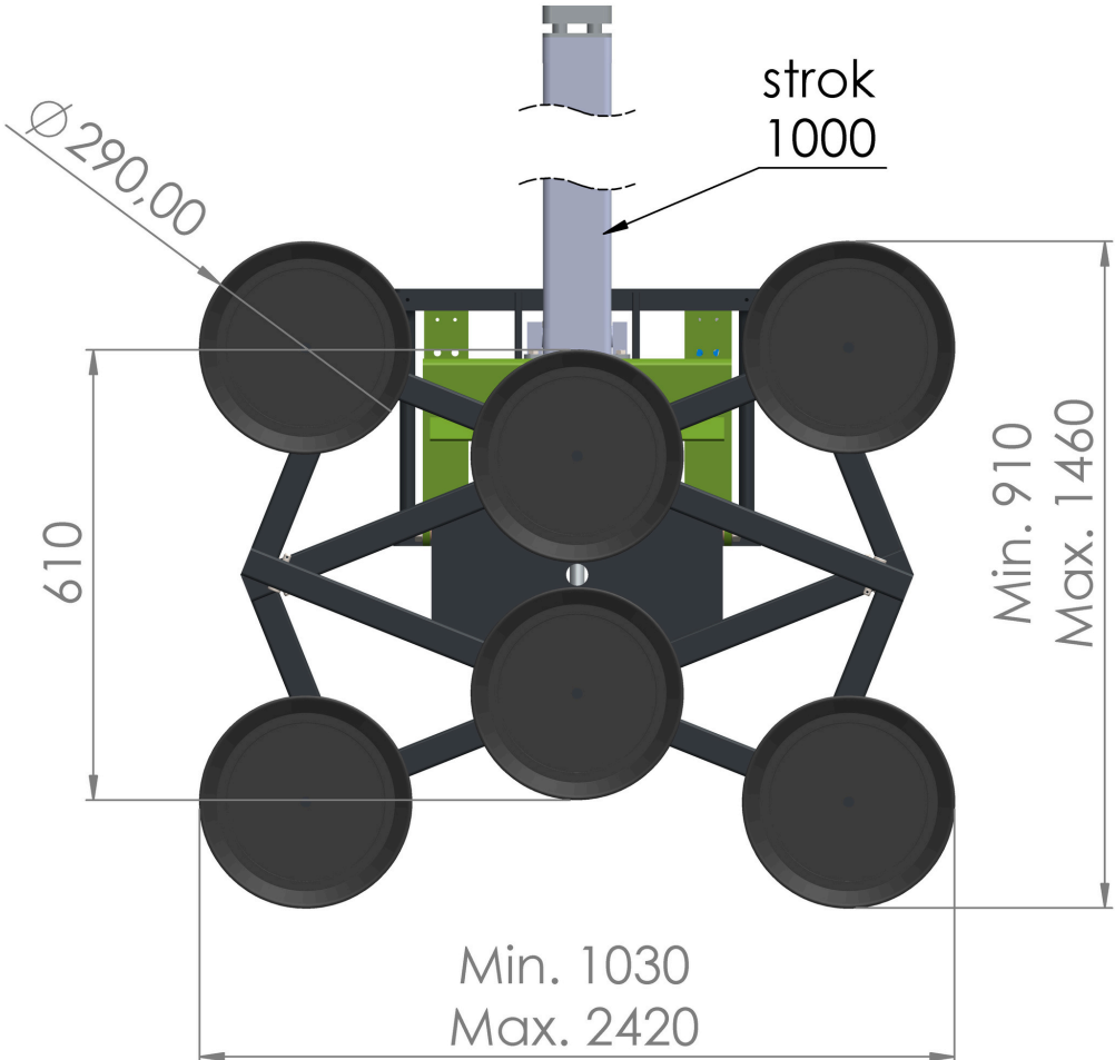
PVL-600VT-EW Lifting with electric winch
