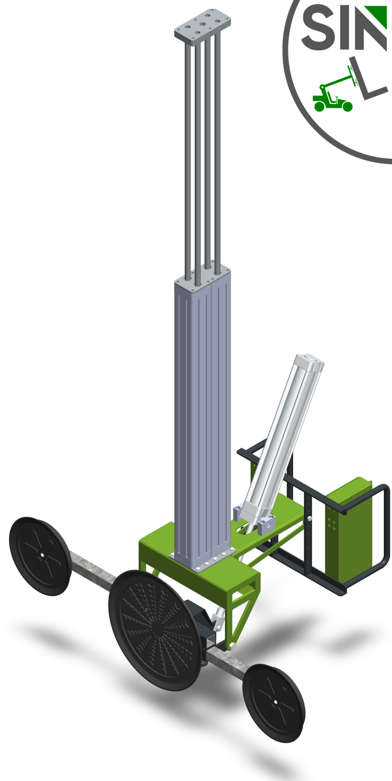
PVL-300VT-PL Lifting with pneumatic cylinder
