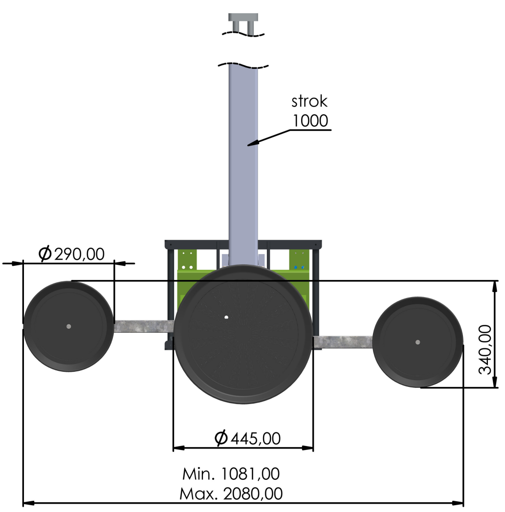
PVL-300VT-EW Lifting with electric winch
