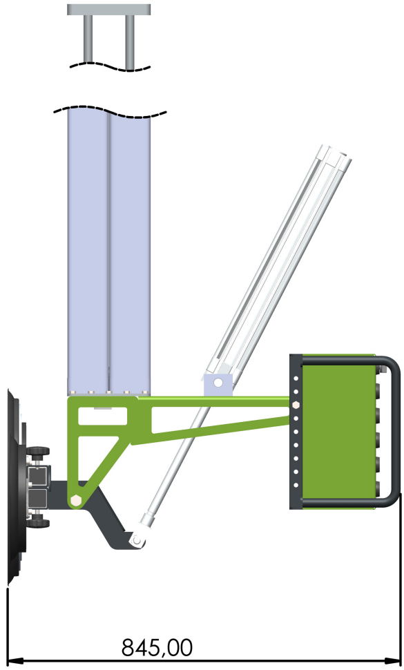
PVL-300VT-PL Lifting with pneumatic cylinder
