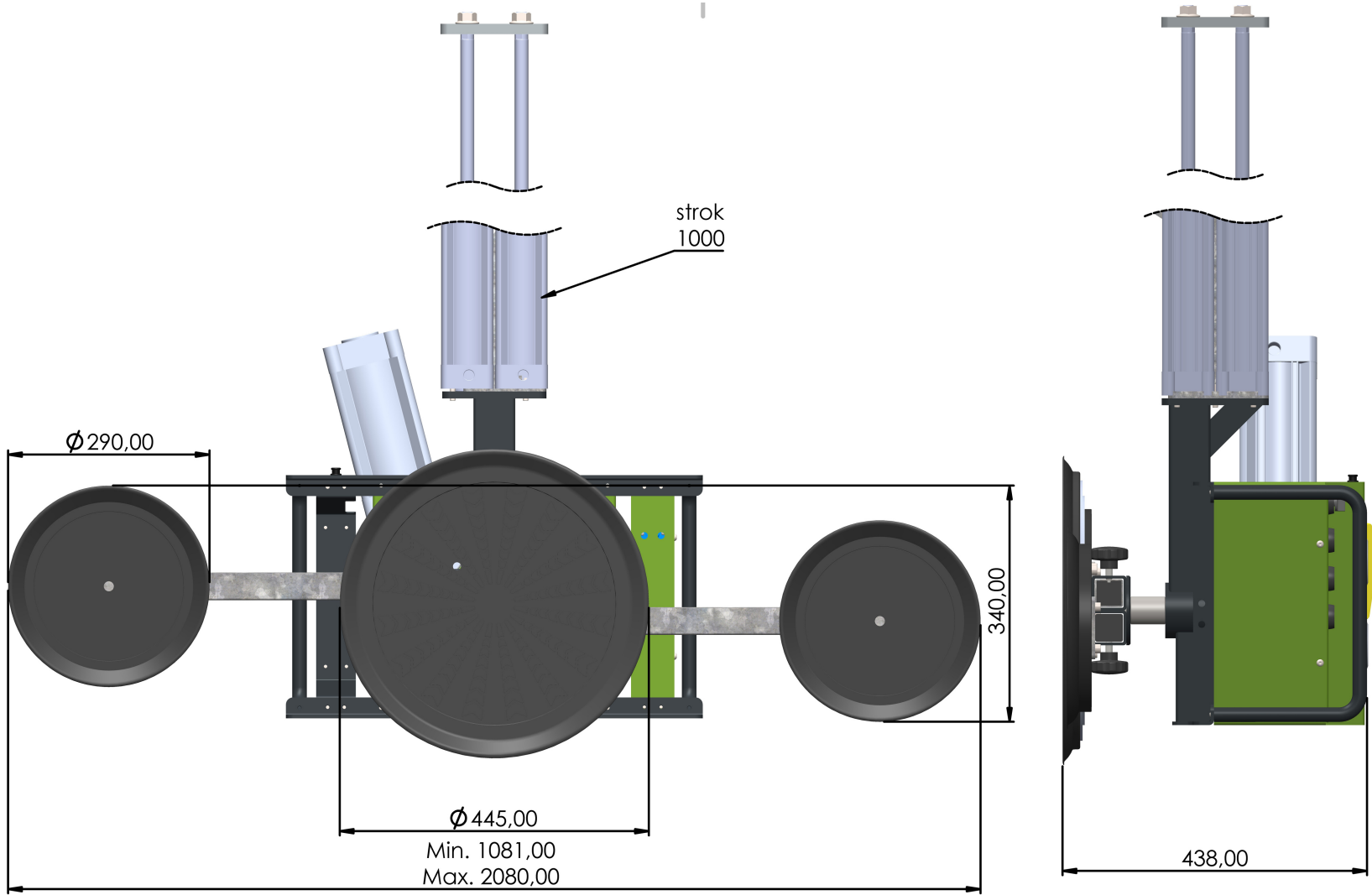
PVL-300VR-EW Lifting with electric winch
