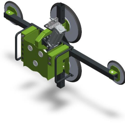
SL-PVL-500VR/EW Lifting with an electric winch
