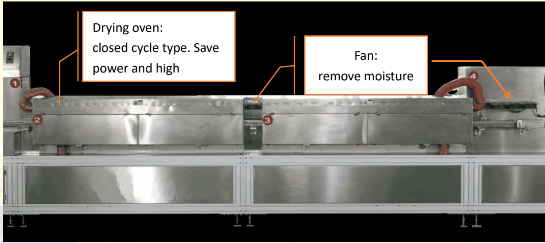
The drying chain sending the swabs to drying oven.
