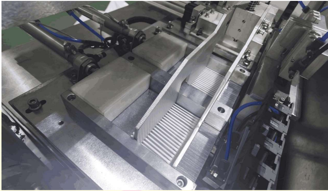
The suction will put and gather swab at here of packing table.
