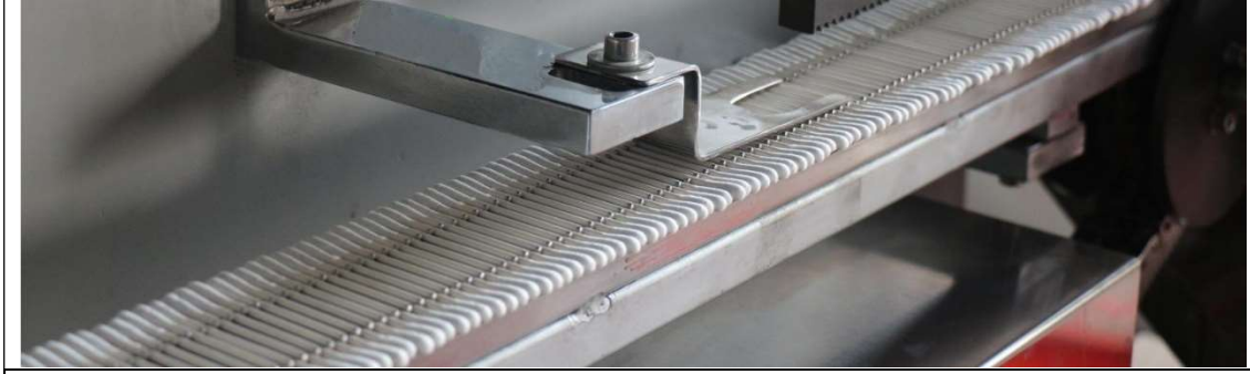
The drying chain sending the swabs to drying oven.
