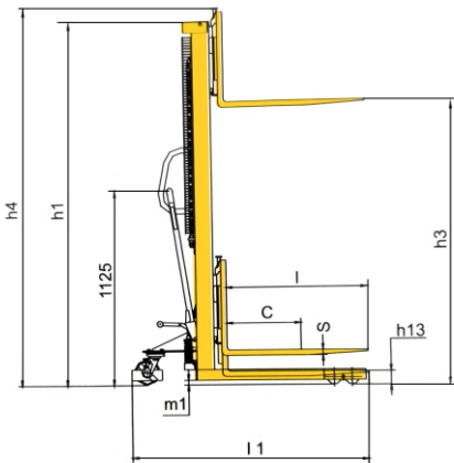
MS SERIES WITH ADJUSTABLE FORKS
