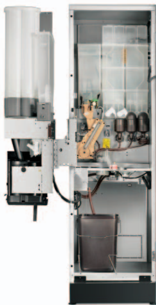
Optimum internal access Z 3000 patented coffee group
