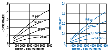
Output Power vs. Speed
