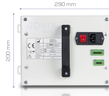
CONNECTION PANEL
