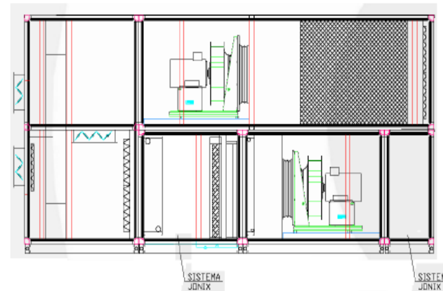
AIR HANDLING UNIT
