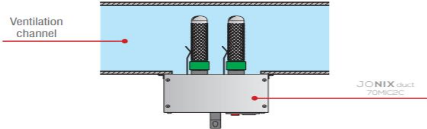
Fastening example of the JONIX duct module on ventilation pipes.
