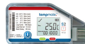
Main Technical Specifications tempmate.®-S2 TH
