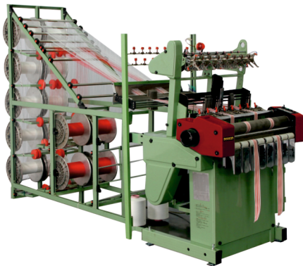
JYF5 8/55 - Double roller needle loom
